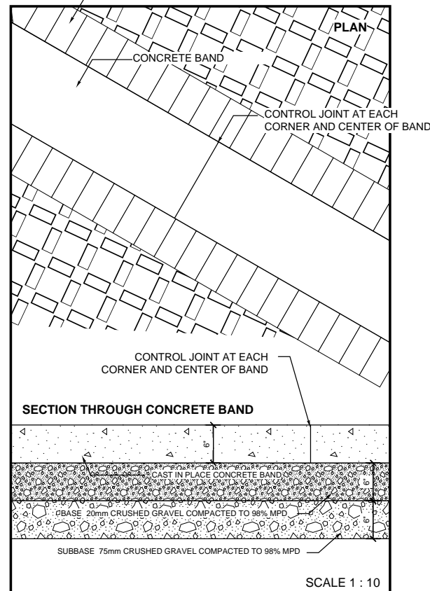
CONCRETE PAVER WITH CONCRETE BAND BETWEEN PAVER BLOCK DETAIL
