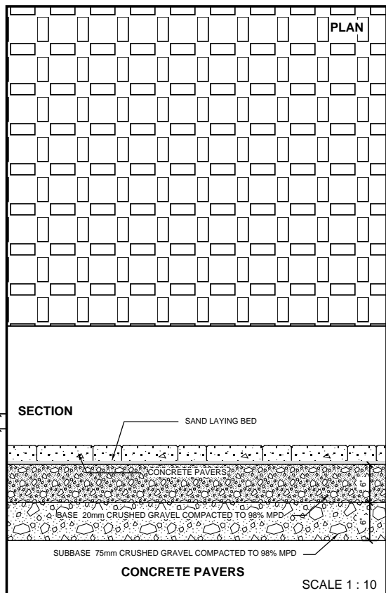
CONCRETE PAVER IN WALKWAY/DRIVEWAY DETAIL
