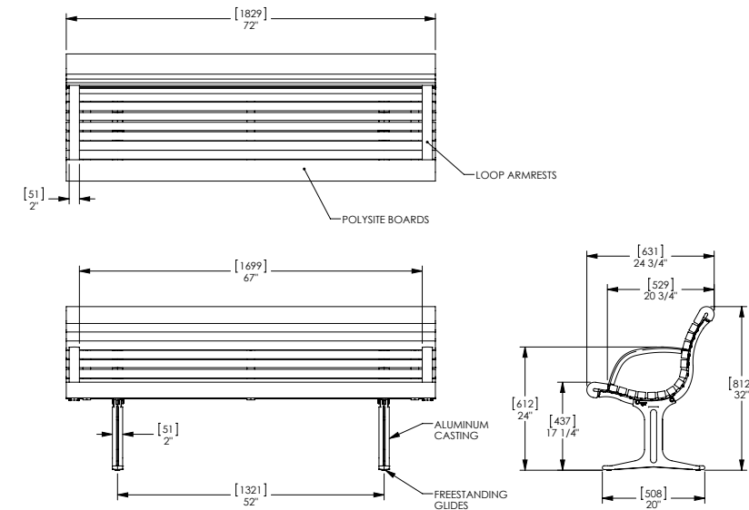
landscapelforms Drawing: GF133-08 Dimensions are in inches (mm)
