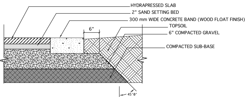
TYPICAL SECTION THROUGH PAVING EDGE
