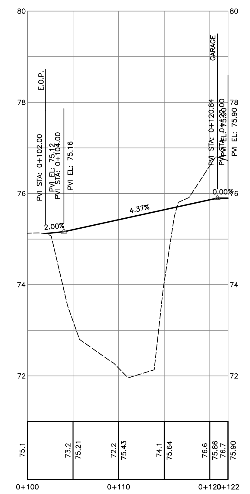
LOT 3 DRIVEWAY PROFILE
