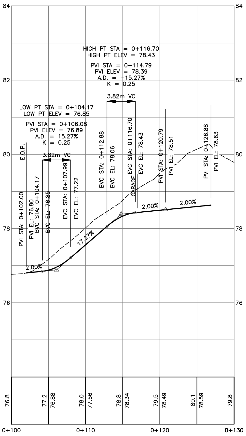
LOT 2 DRIVEWAY PROFILE
