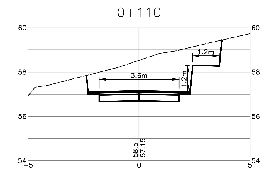
SECTIONS 1:100
