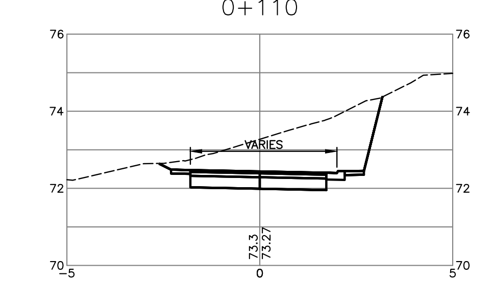
SECTIONS 1:100
