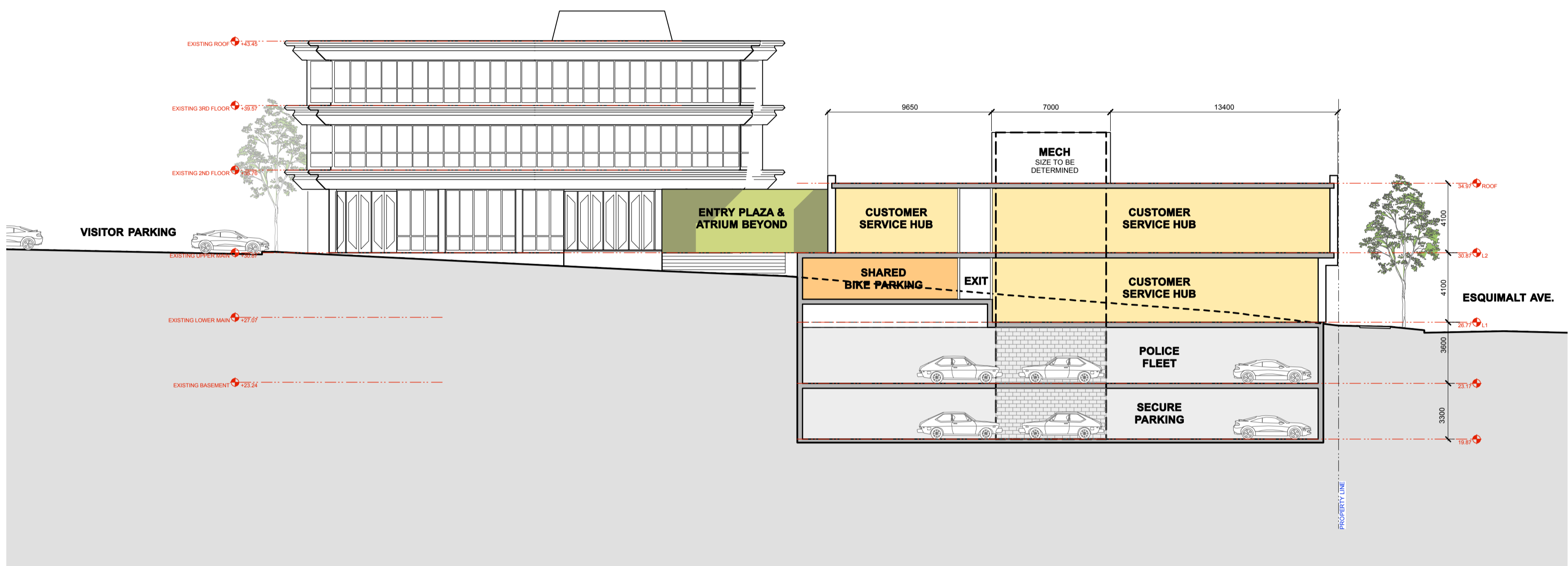
North/South Section (Looking East)
