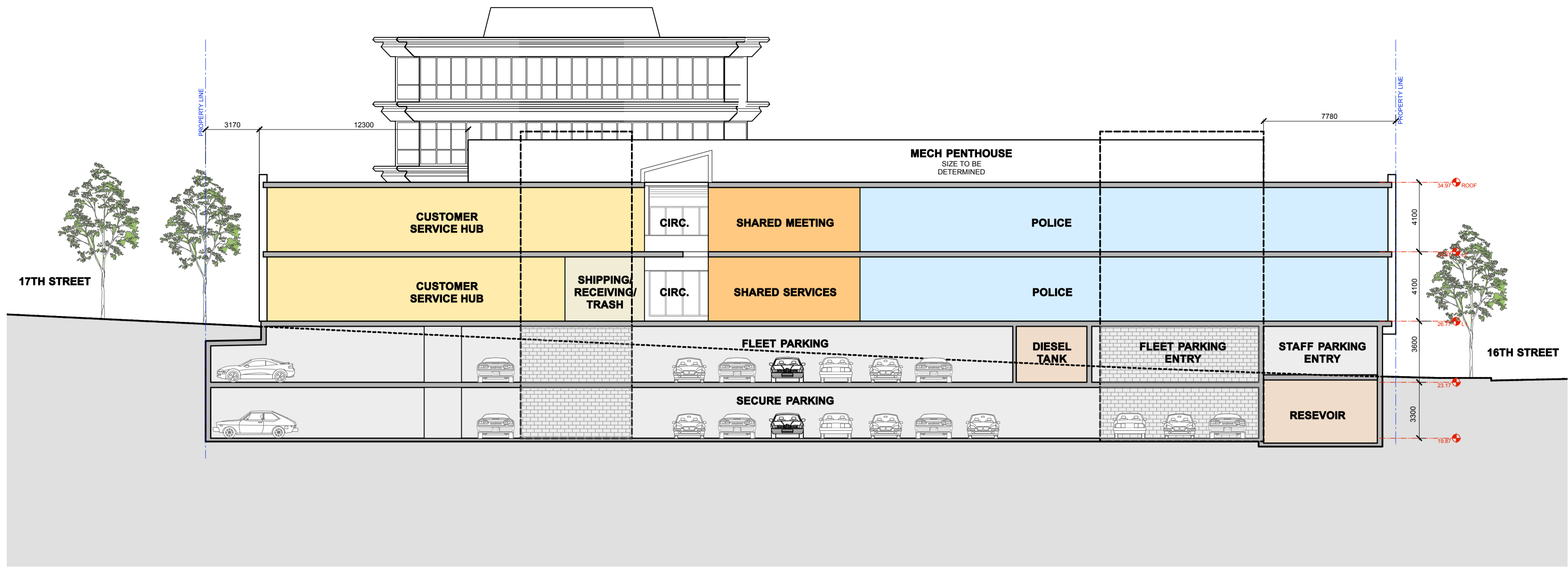
East/West Section (Looking North)
