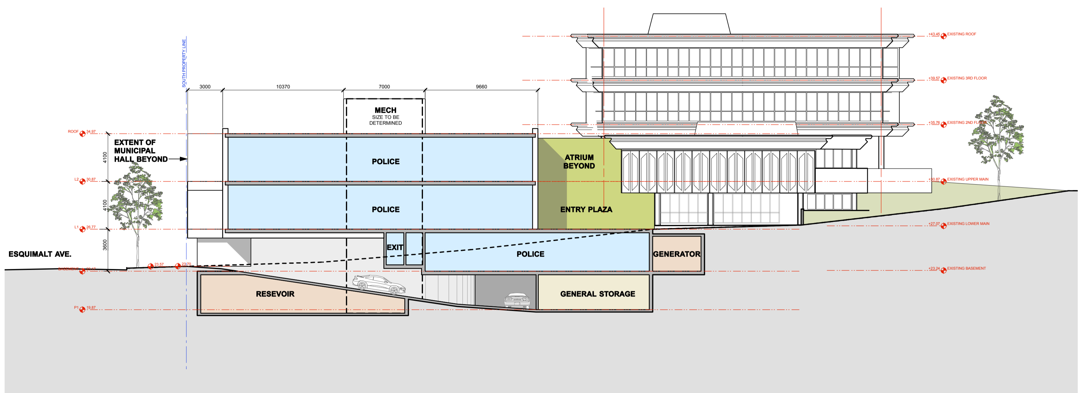
North/South Section (Looking West)
